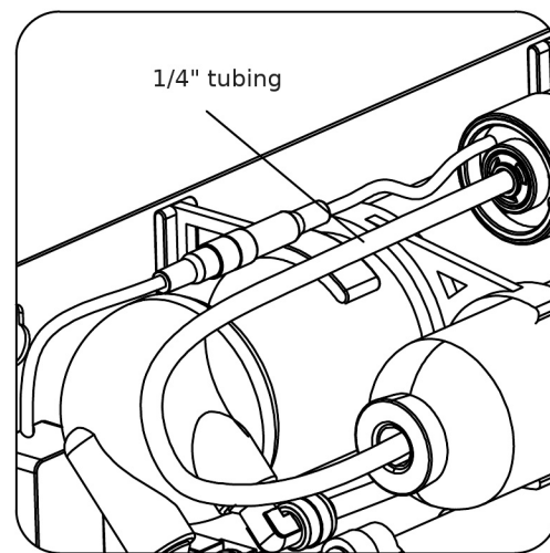
6. Connect the tubing between the post-carbon filter and sterilizer.
