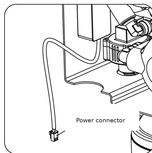
8. Connect the sterilizer power connector to the water purifier control circuit.
