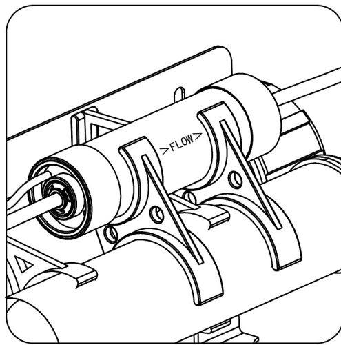
3. Secure the other side of the double clip to the post-carbon filter.
